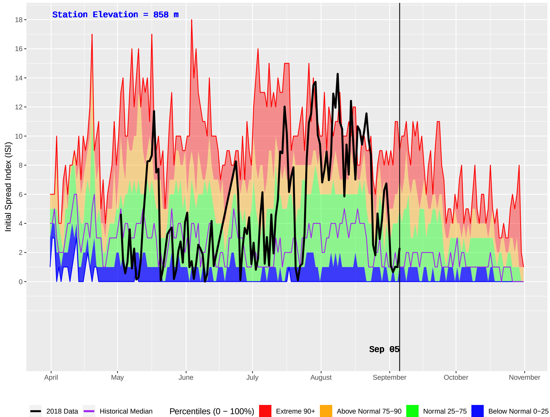
BEDNESTI (175) : Historical (1993–2016) and Current (2018) Daily Initial Spread Index (ISI)
