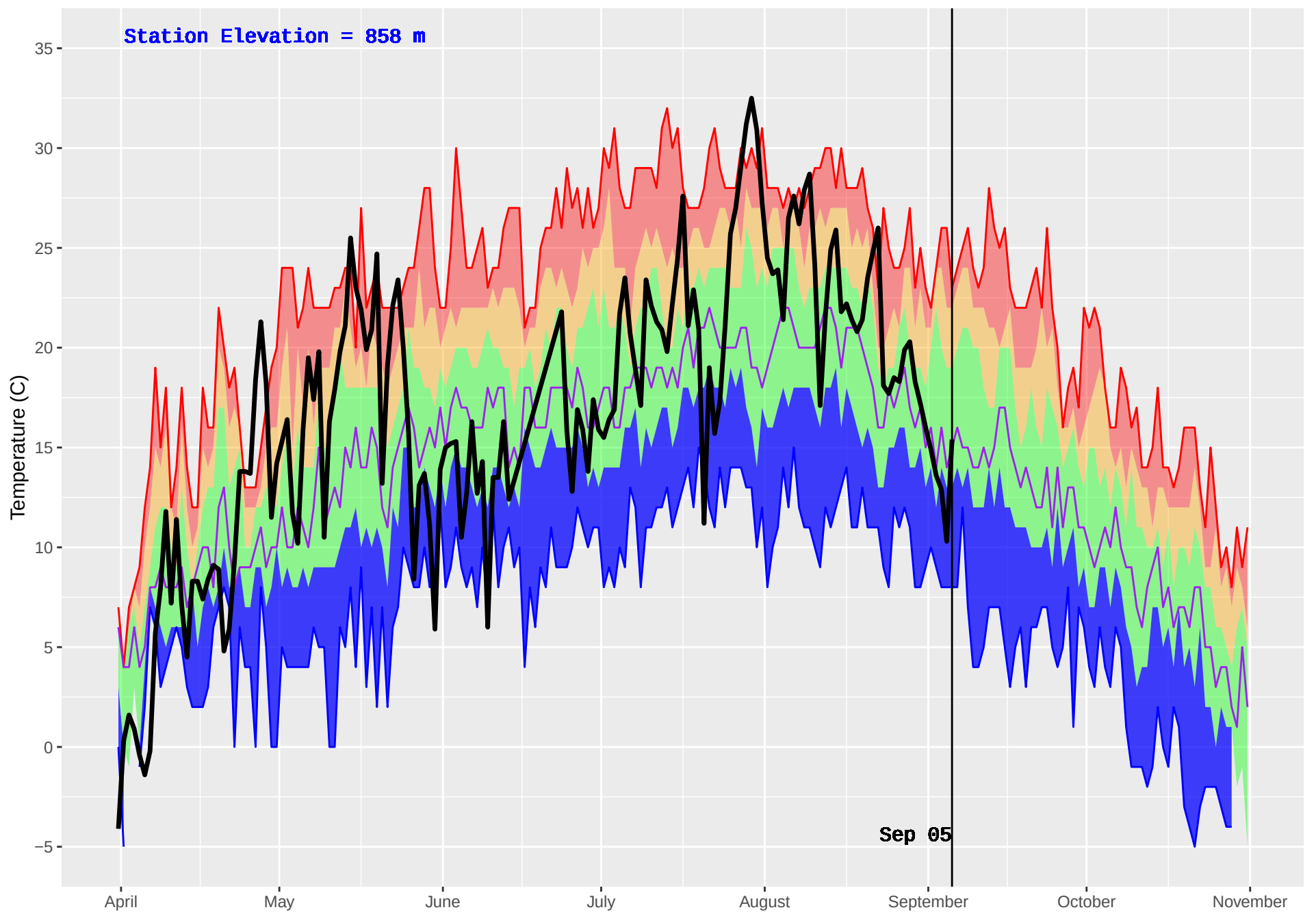
BEDNESTI (175) : Historical (1993–2016) and Current (2018) Daily Temperature
